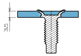
Section View A-A After Placing
