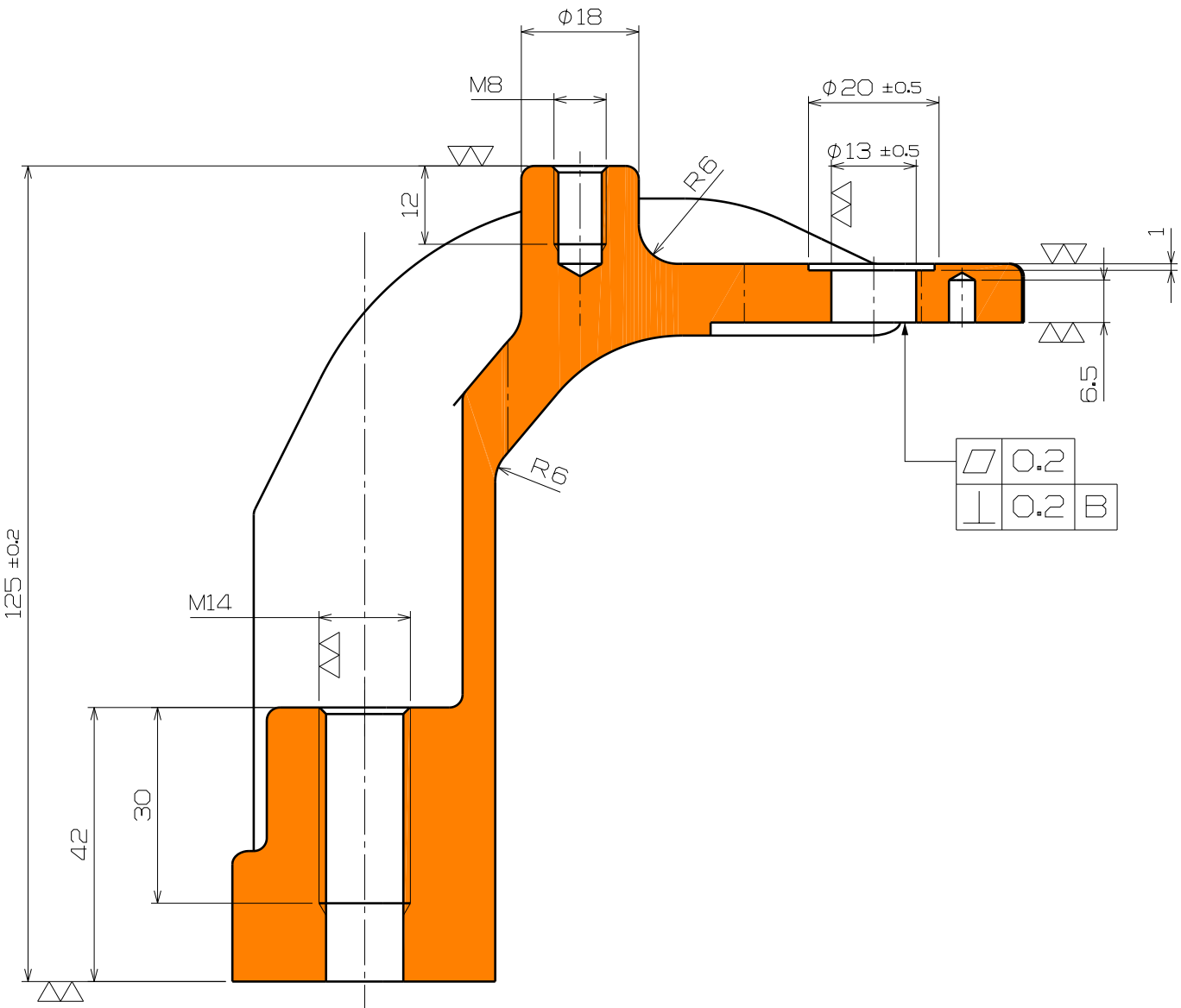
Section View A-A
