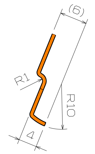
Section Cut E-E
