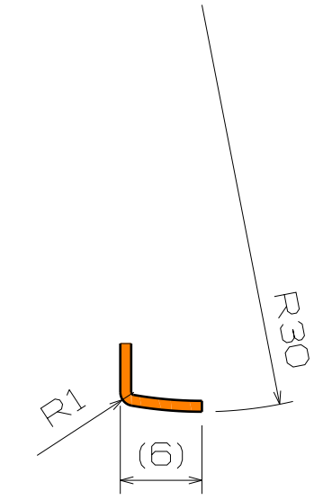
Section Cut G-G
