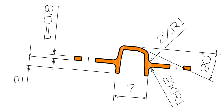
Section Cut B-B
