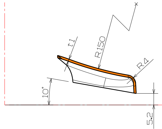
Section View H-H
